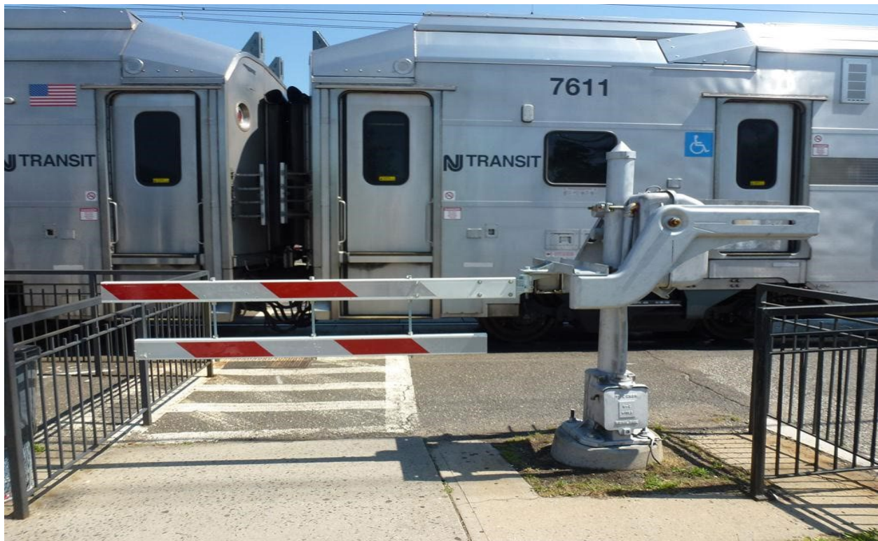
Figure 1. Example of a pedestrian gate skirt with sidewalk fencing at a grade crossing in Matawan, NJ Image Credit: Volpe Center
